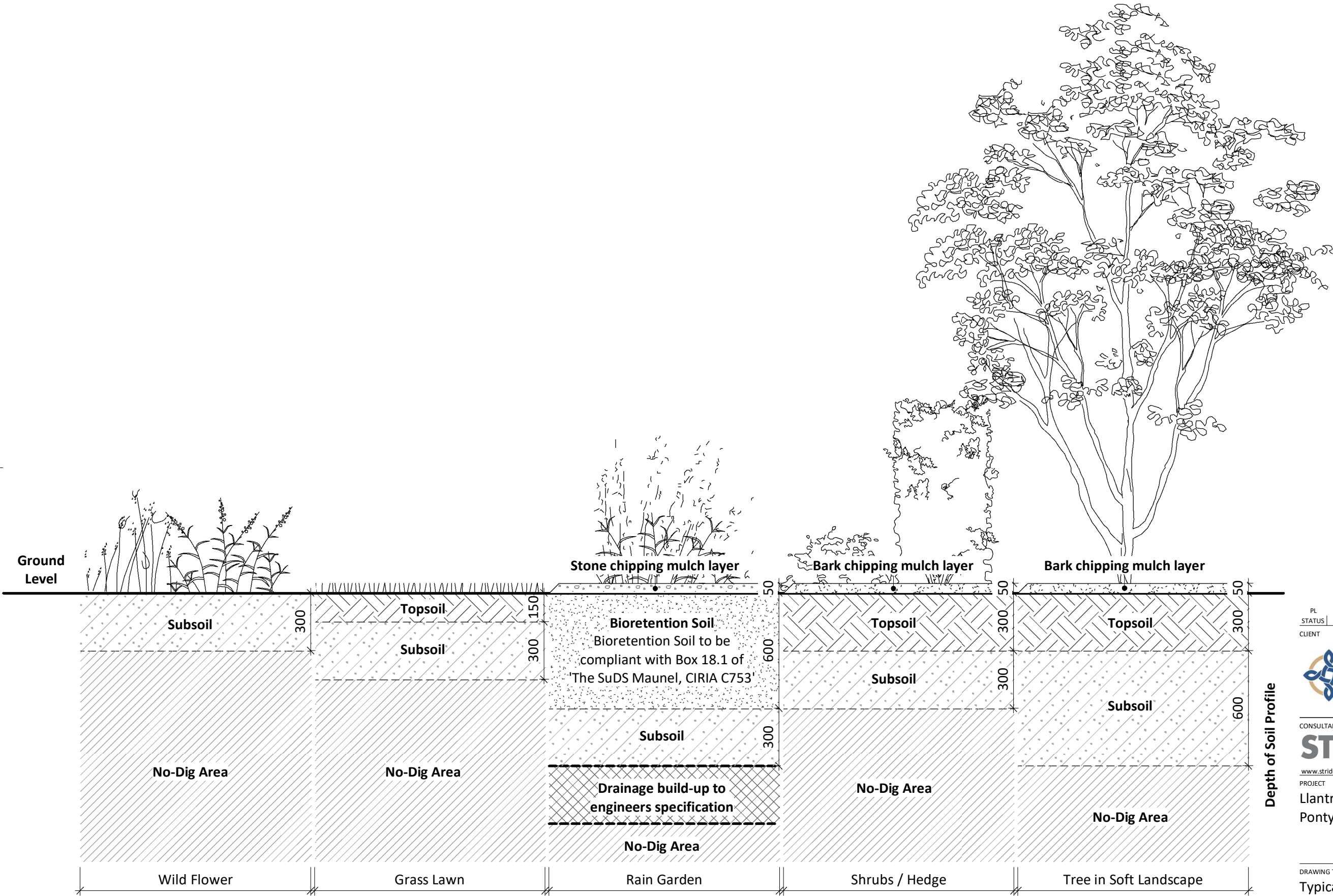
Typical Soil Profile for Soft Landscape 1 : 20
