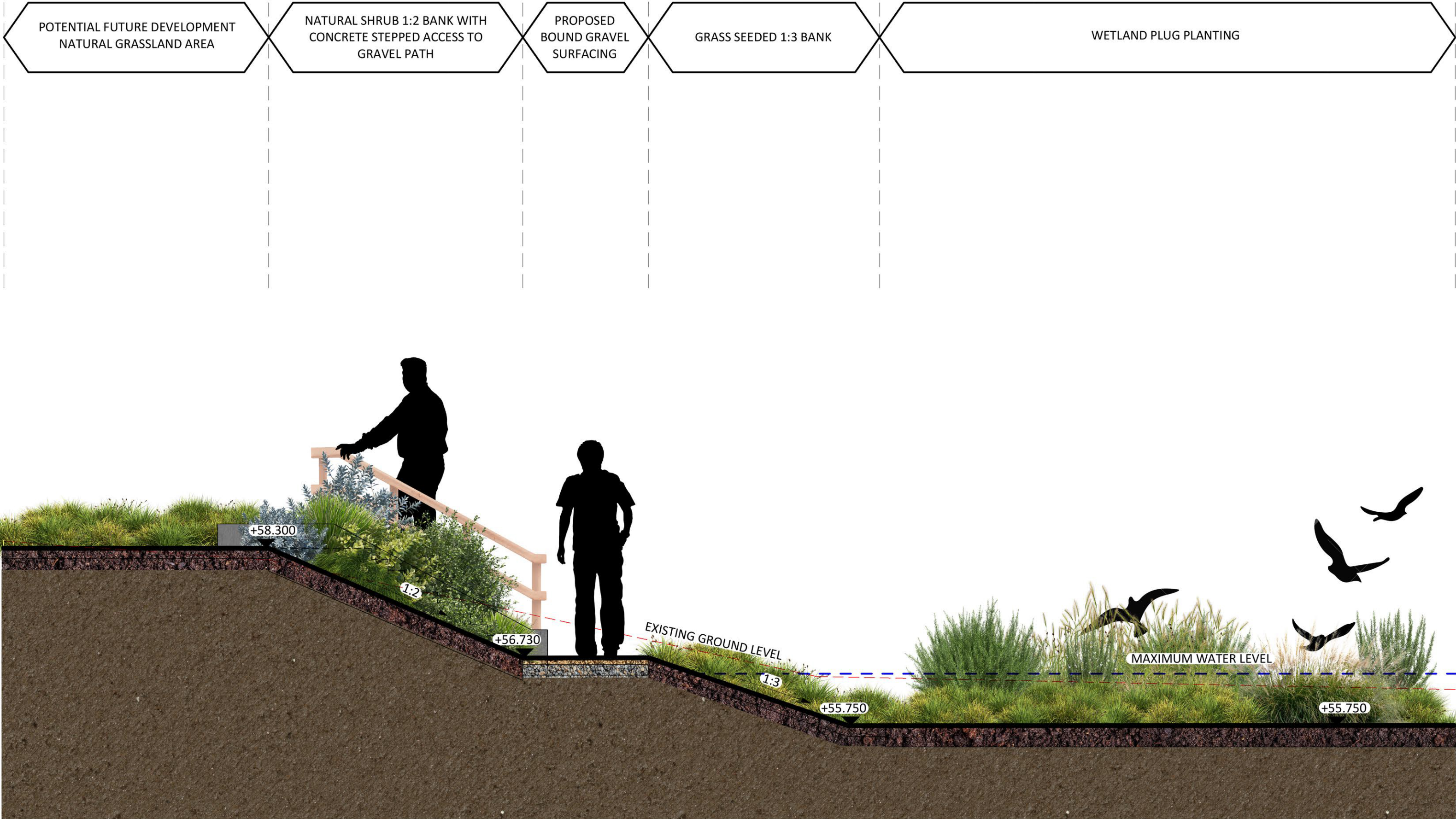
92050 Section A 1:50
