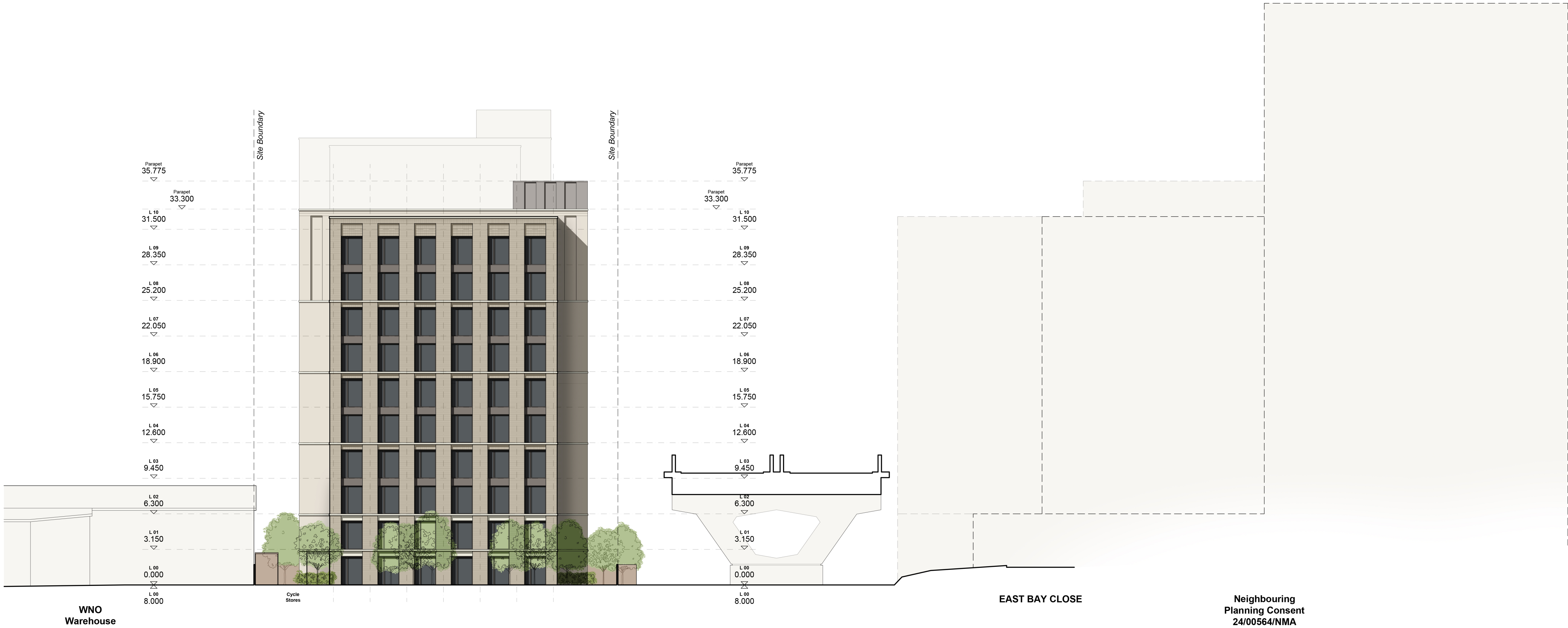
Proposed Elevation 04 - South Facing (Tyndall Street) Scale 1:200 at A3
