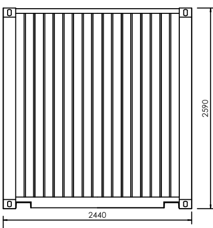
20ft Shipping Container - Front Elevation
