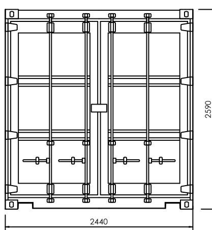
20ft Shipping Container - Door Elevation
