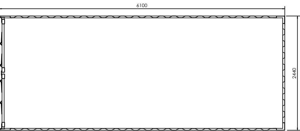
20ft Shipping Container - Plan View
