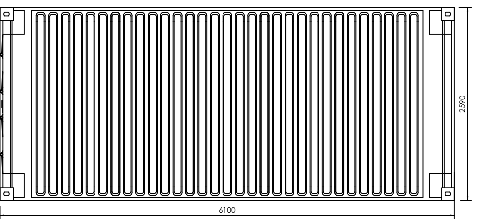
20ft Shipping Container - Roof Plan
